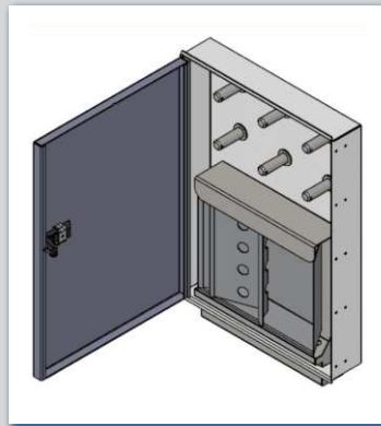
Gear & Tray Cabinet - Holds 3 Gear Sets - Includes Removable Sump to Catch Oil
