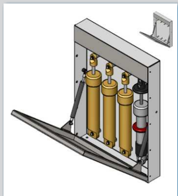
4 Position Shock Cabinet - Shocks are NOT Included
